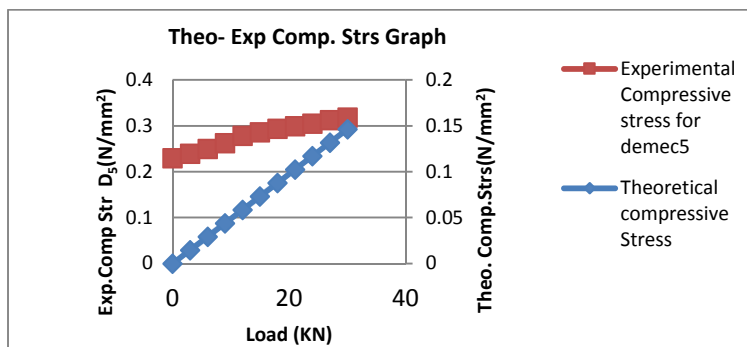
Figure 3.4 Load Against compressive Stress for Demec 1,3 & 5
